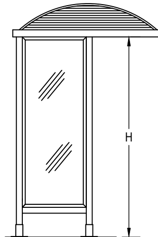
FRONT ELEVATION
